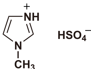
1-Methylimidazolium Hydrogen Sulfate
