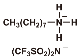
n -Octylammonium Bis(trifluoromethanesulfonyl)imide
