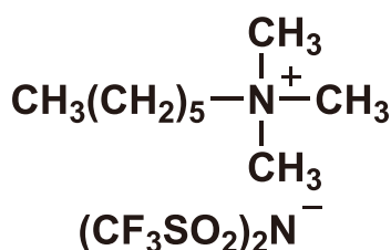
Trimethylhexylammonium Bis(trifluoromethanesulfonyl)imide
