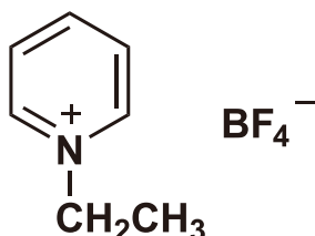
1-Ethylpyridinium Tetrafluoroborate
